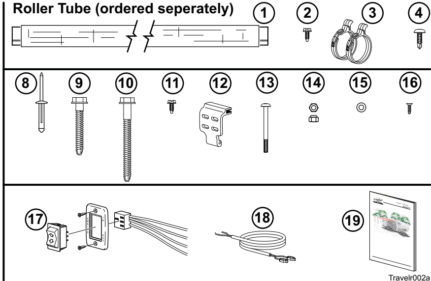
Figure 2. Component Checklist.
