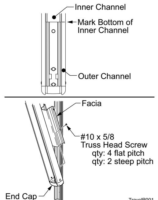
Figure 14. Attaching the Fascia.
